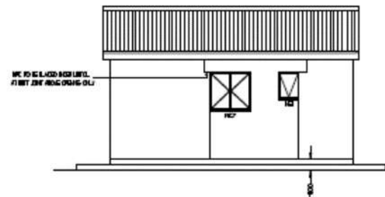
ELEVATION - 2 SCALE 1:50
