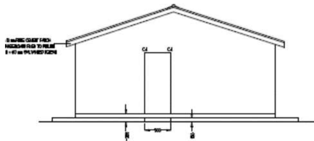
ELEVATION - 1 SCALE 1:50
